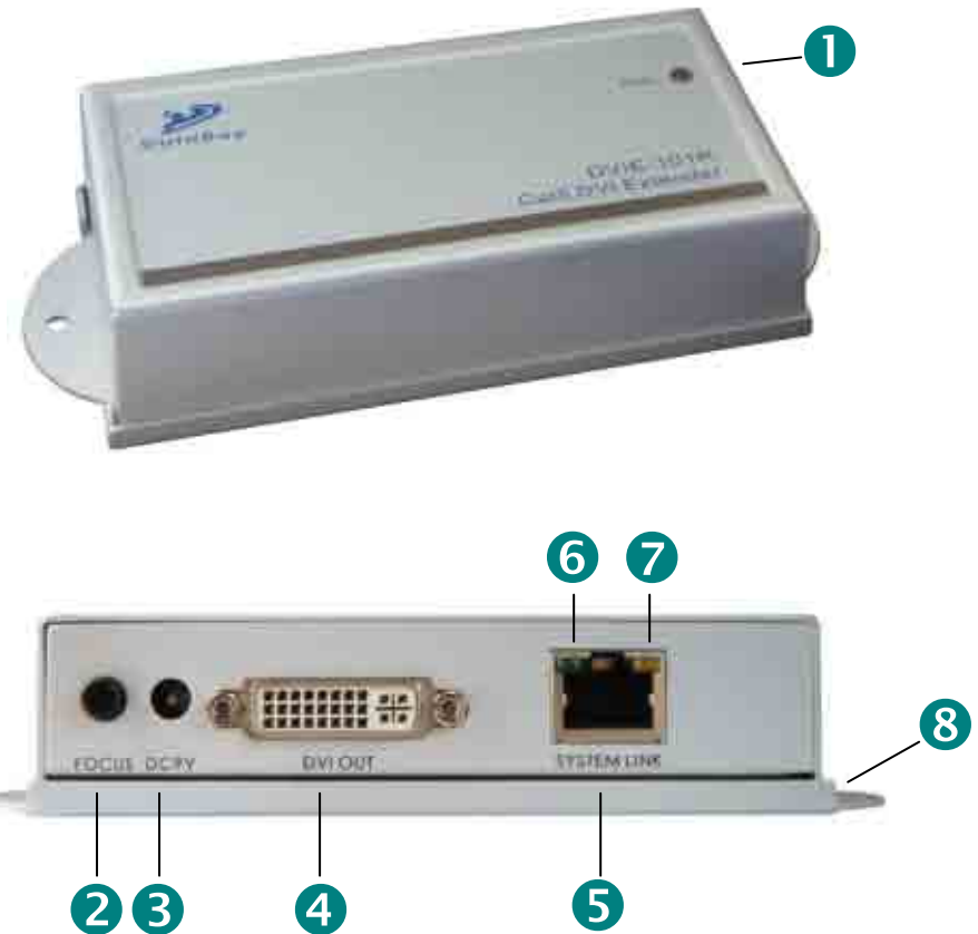
DVIE-101R DVI-D Long Range Receiver
